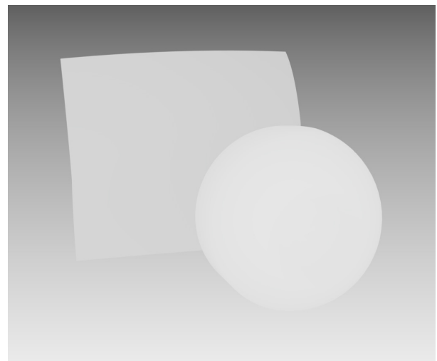
Rendu Z-buffer.
