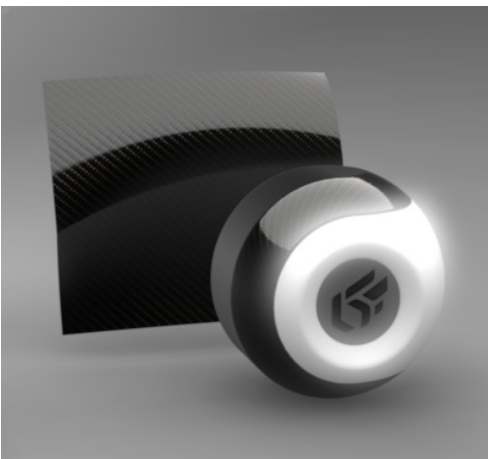
Bloom.
