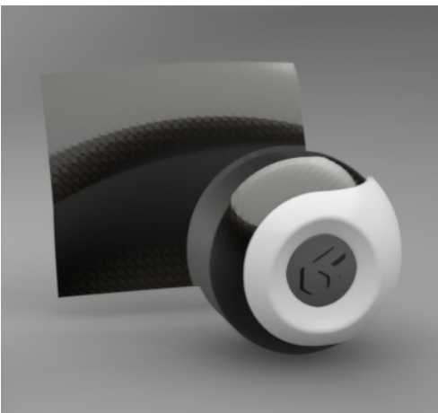
Dilatation.
